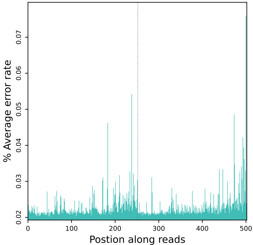
Error rate distribution along reads (R10415)
